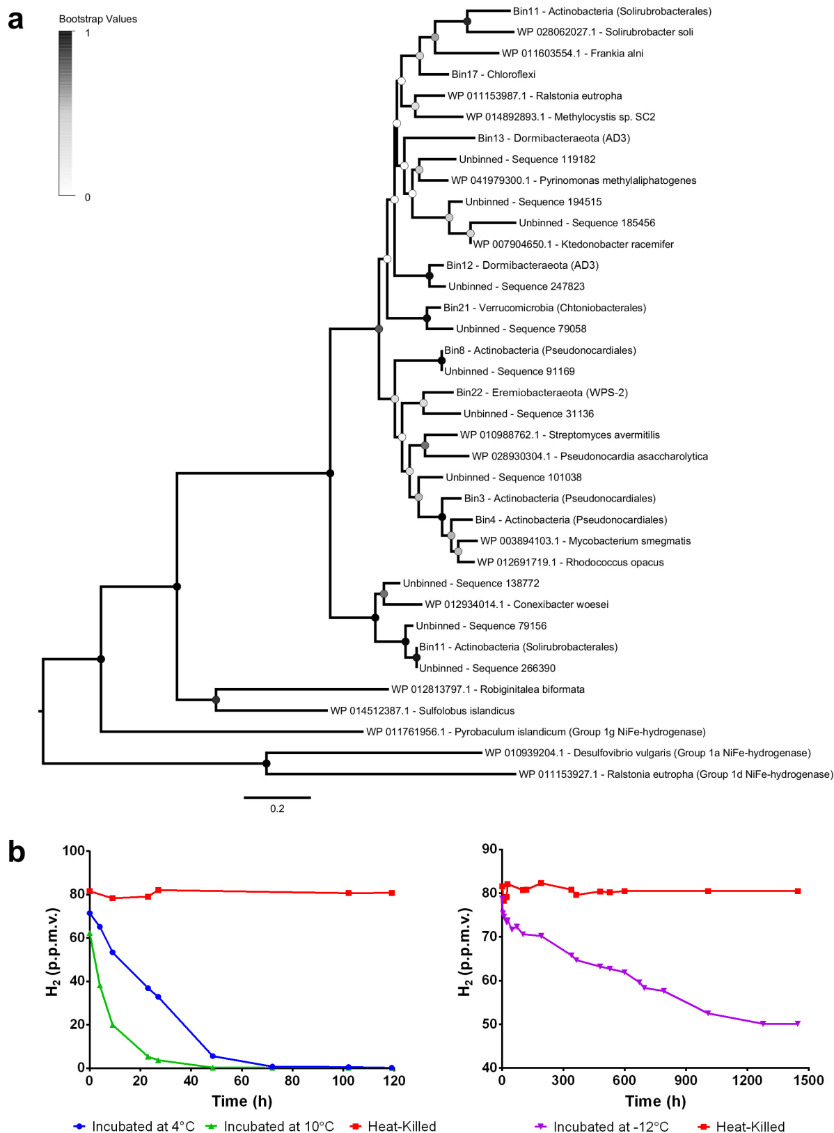
Extended Data Figure 5 | Amino acid phylogeny and inferred activity of hydrogenase enzymes in sampled soils. a , Expanded phylogenetic tree of [NiFe]-hydrogenase large subunit genes retrieved from the Robinson Ridge metagenome data. The phylogenetic tree was generated by the maximum-likelihood method and robustness was tested with 500 replicates. Hydrogenase genes were common within the metagenome and
