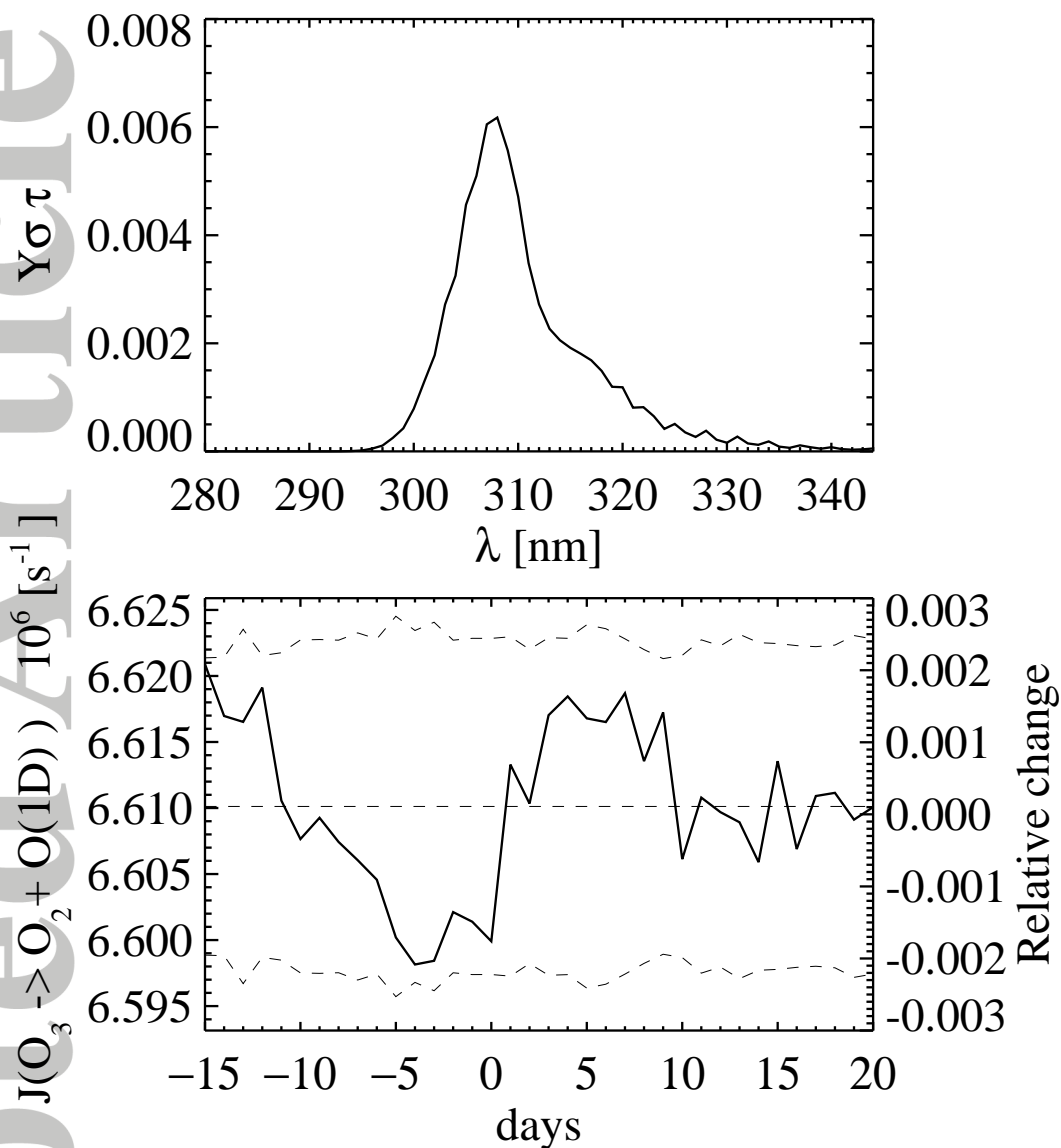
Figure 13. Top panel: The wavelength range where the reaction \text{O}_3 + \gamma \rightarrow \text{O}_2 + \text{O}(1\text{D}) can occur in the lowest part of the atmosphere. The relatively narrow shape is a result of the atmospheric transmission \tau(\lambda) cutoff at shorter wavelengths and the cross-section \sigma(\lambda) cut-off at longer wavelengths. Bottom panel: Composite change in the photolysis constant for the reaction in Eq. 33, for the three largest FDs in the interval 2003-2006. Although there is a decrease in J , the change is only of the order 2\text{-}3 \times 10^{-3} . The dashed lines are the 1-\sigma variance.
