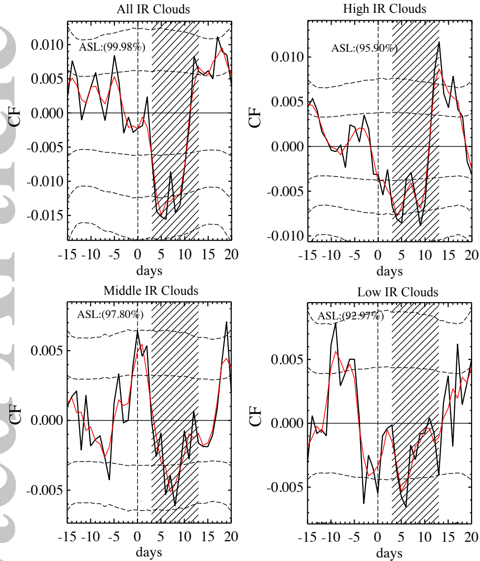
Figure 7. Statistics of IR detected ISCCP cloud fractions averaged over the oceans for the five strongest FD after 1998. The red curve is a 3-day smoothing of the daily data. Top left panel: All IR detected clouds. Top right panel: High clouds. Bottom left panel: Middle clouds. Bottom right panel: Low clouds. The hatched area denotes the temporal interval used to integrate the response (3-13 days) and the achieved significance levels is stated in each panel. The dotted lines are one, two, and three standard deviations obtained using the MC bootstrap analysis.
