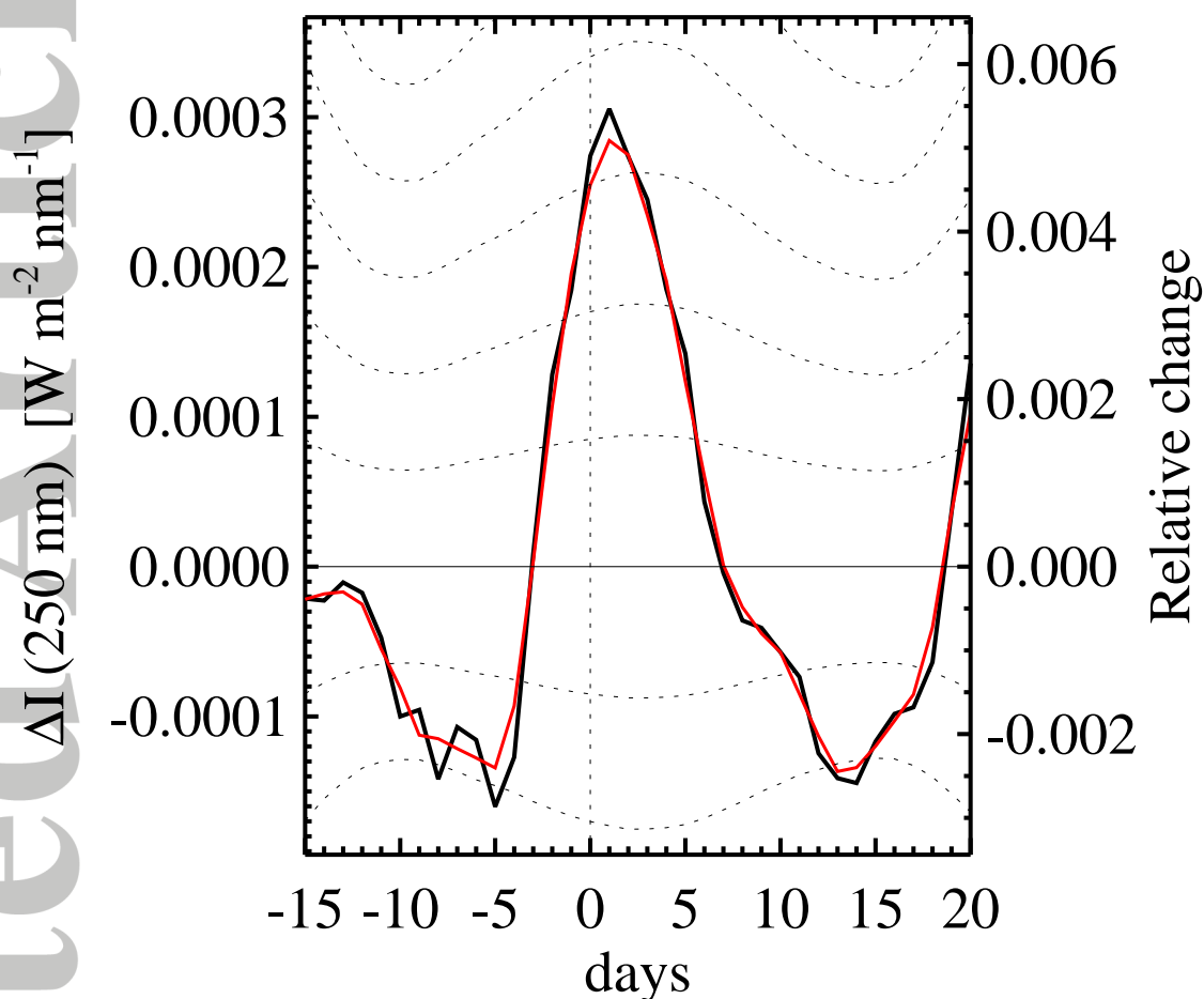
Figure 14. UV variation at \lambda = 250 nm superposed and centred at the 3 strongest FD after 2003 (data from FD 2 and FD 5 from table 1 are not available in the SORCE data set). Notice the that the relative change is of the order 0.8 %. The maximum seen in UV is due to the rotation of active regions with a period of ca. 27 day (see also Fig. 15). Typically an active region at maximum UV and a FD are closely correlated since a CME has to hit the Earth to generate a significant FD. The dashed lines are the n\text{-}\sigma variance, n=1,2,\dots .
